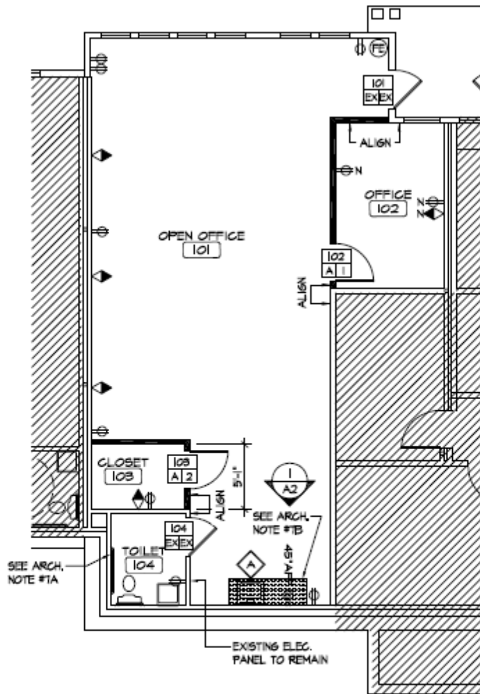
2 ARCHITECTURAL & POWER PLAN A1 SCALE: 1/8" = 1'-0"
