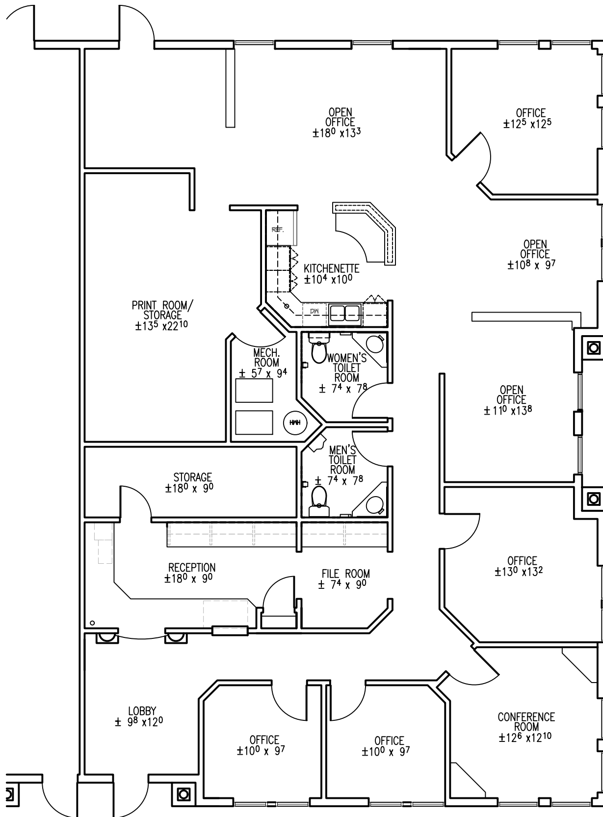
EXISTING FLOOR PLAN SCALE: 1/8" = 1'-0"
